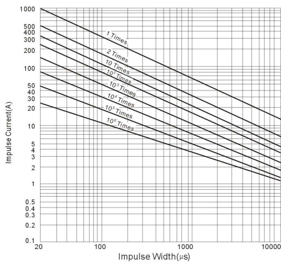
Surge Life Reting [180KD 14 to 680KD 14]
