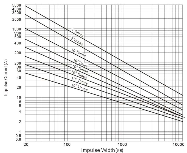
Surge Life Reting [820KD 14 to 182KD 14]
