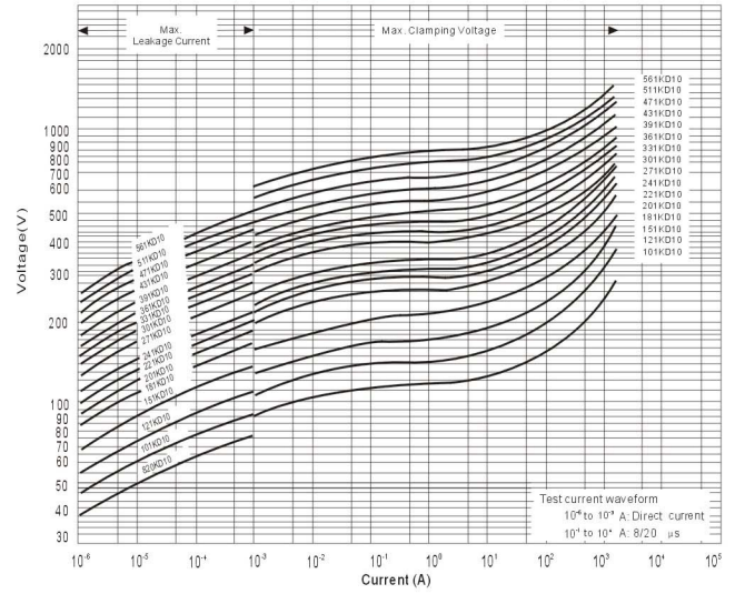
V-I Curve [820KD10 to 561KD10]
