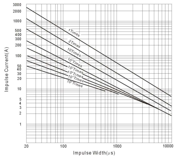
Surge Life Time Reting [820LD10 to 112KD10]
