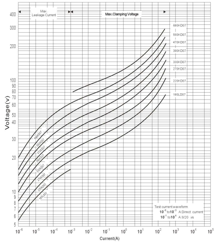
V-I Curve[180LD07 to 680KD07]
