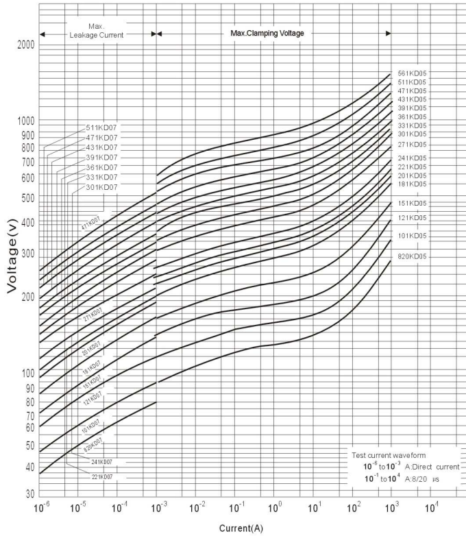
V-I Curve[820KD07 to 560KD07]
